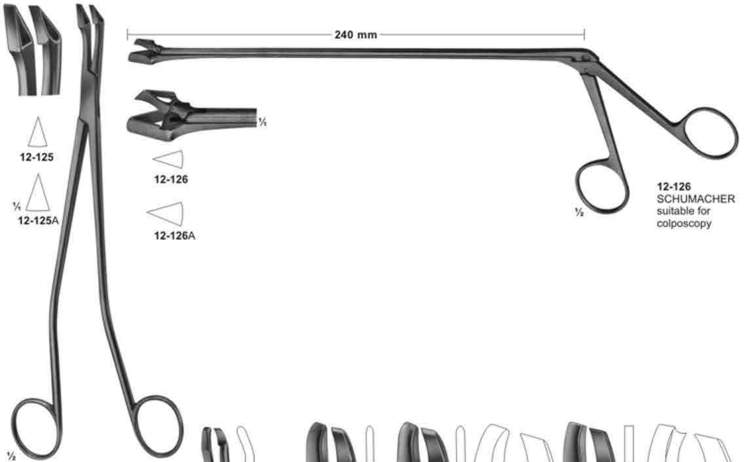
12-125 SCHUMACHER 240mm
